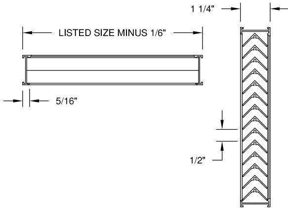
MODEL - DGC - FLANGLASS FRAME
